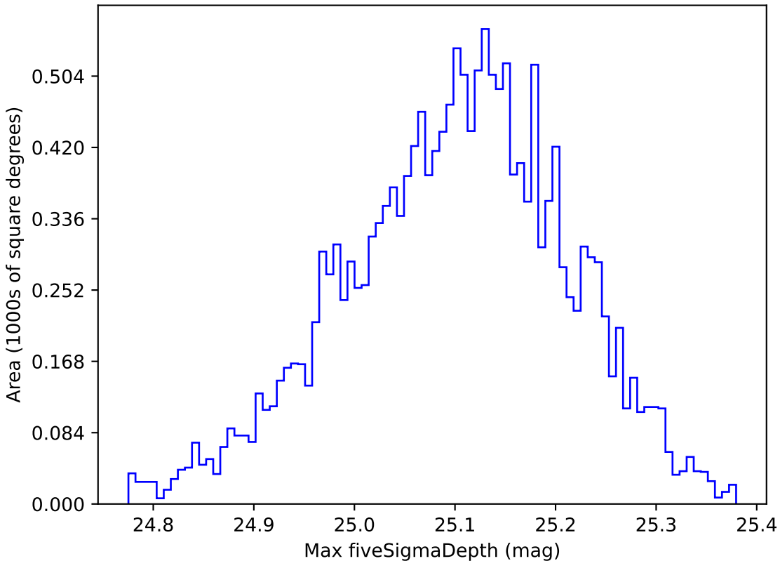
ddf_loaded_fl1_v3.4_10yrs WFD g band: Max fiveSigmaDepth
