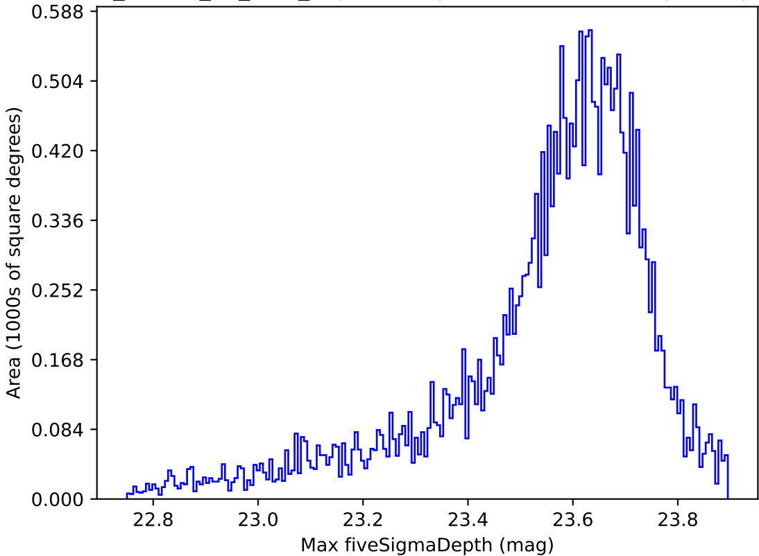
ddf_loaded_fl1_v3.4_10yrs All sky z band: Max fiveSigmaDepth
