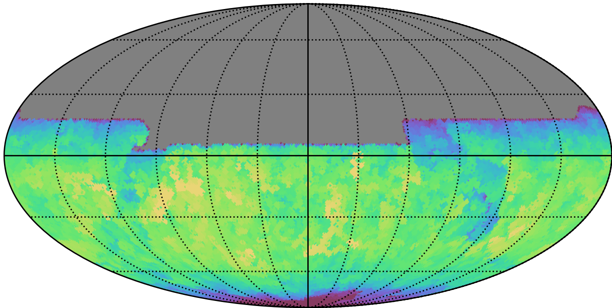
ddf_loaded_fl1_v3.4_10yrs All sky y band: Max fiveSigmaDepth
