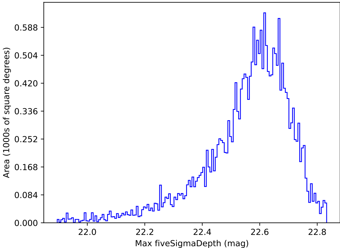
ddf_loaded_fl1_v3.4_10yrs All sky y band: Max fiveSigmaDepth
