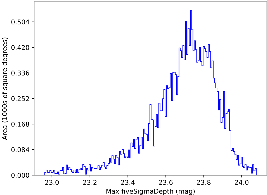
ddf_loaded_fl1_v3.4_10yrs All sky u band: Max fiveSigmaDepth
