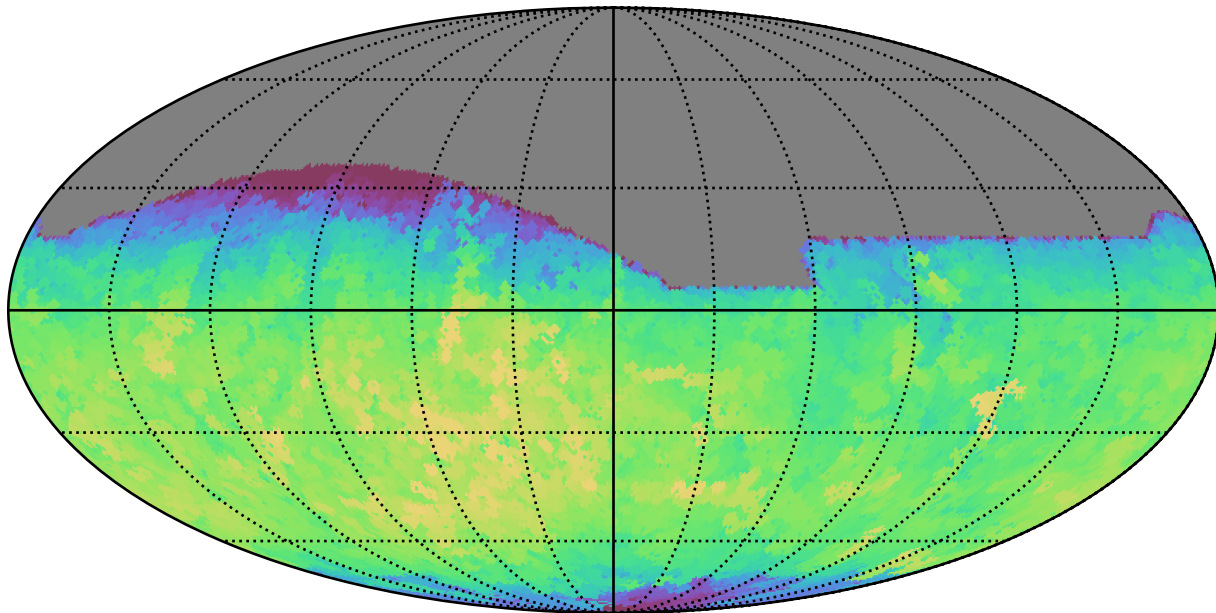
ddf_loaded_fl1_v3.4_10yrs All sky r band: Max fiveSigmaDepth
