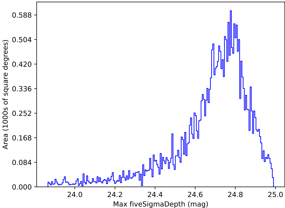
ddf_loaded_fl1_v3.4_10yrs All sky r band: Max fiveSigmaDepth
