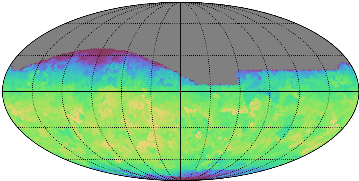
ddf_loaded_fl1_v3.4_10yrs All sky i band: Max fiveSigmaDepth
