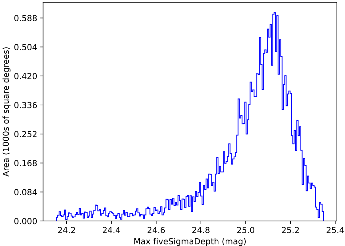
ddf_loaded_fl1_v3.4_10yrs All sky g band: Max fiveSigmaDepth
