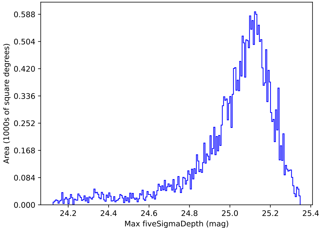
ddf_loaded_fl1_v3.4_10yrs All sky all bands: Max fiveSigmaDepth
