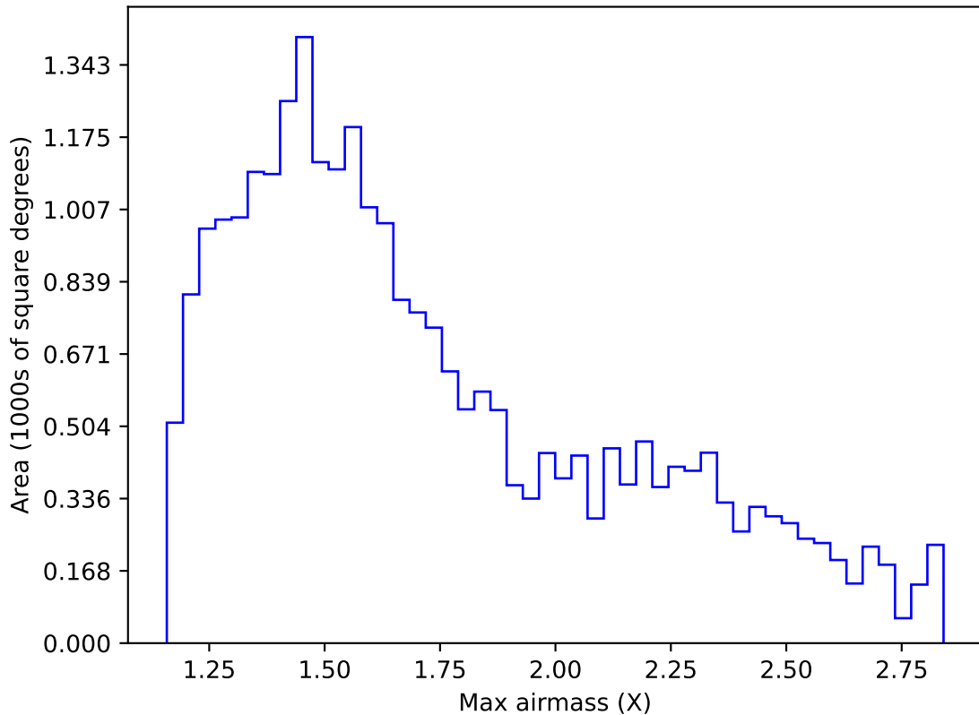
ddf_loaded_fl1_v3.4_10yrs Yr 1 z band: Max airmass
