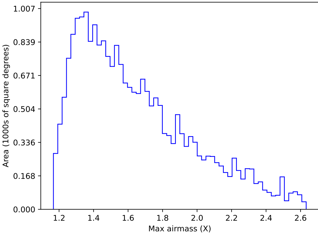
ddf_loaded_fl1_v3.4_10yrs Yr 1 y band: Max airmass
