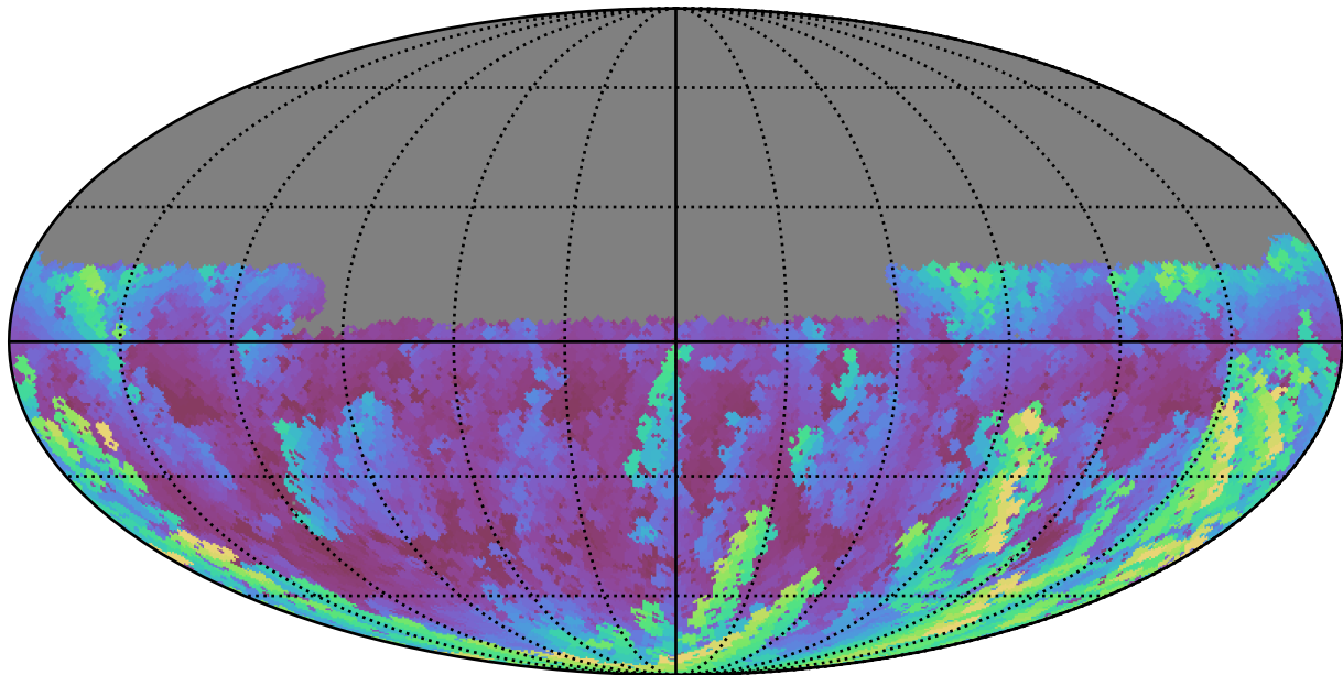
ddf_loaded_fl1_v3.4_10yrs Yr 1 u band: Max airmass
