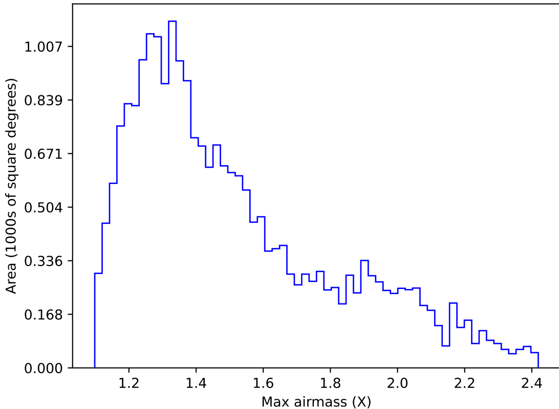
ddf_loaded_fl1_v3.4_10yrs Yr 1 u band: Max airmass
