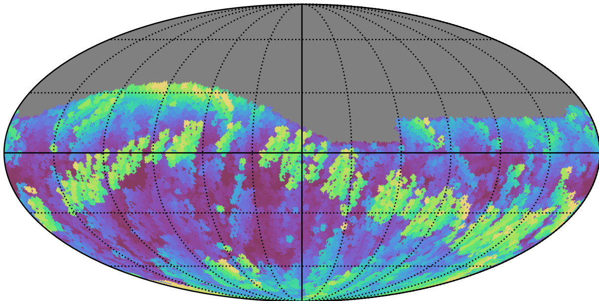
ddf_loaded_fl1_v3.4_10yrs Yr 1 r band: Max airmass
