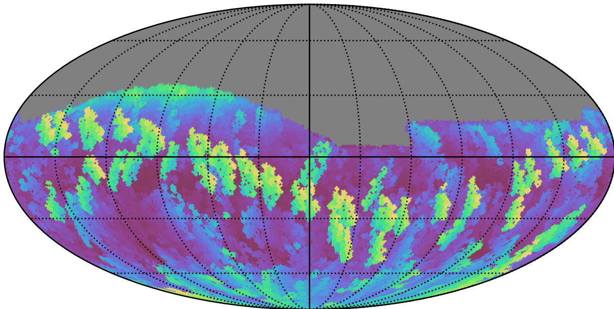
ddf_loaded_fl1_v3.4_10yrs Yr 1 i band: Max airmass
