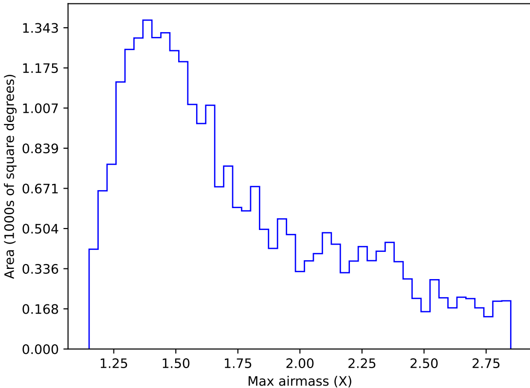
ddf_loaded_fl1_v3.4_10yrs Yr 1 i band: Max airmass
