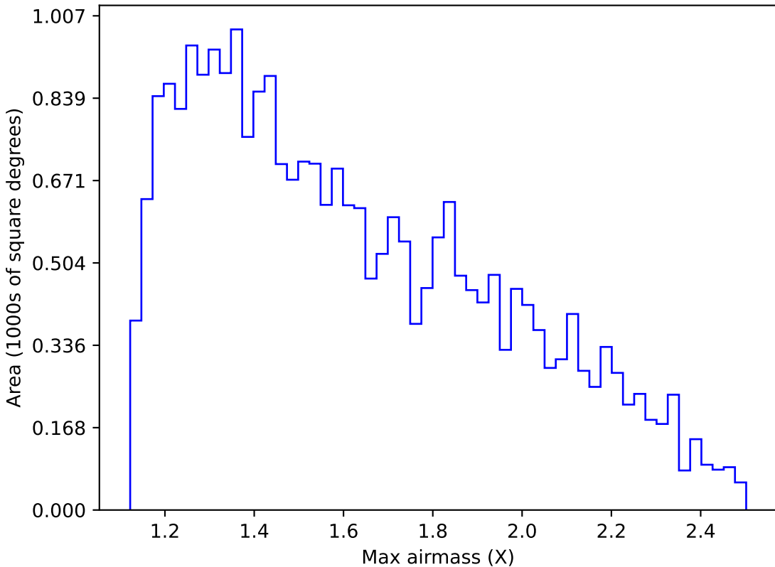
ddf_loaded_fl1_v3.4_10yrs Yr 1 g band: Max airmass
