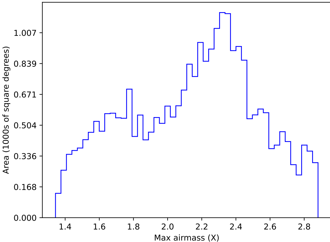
ddf_loaded_fl1_v3.4_10yrs Yr 1 all bands: Max airmass
