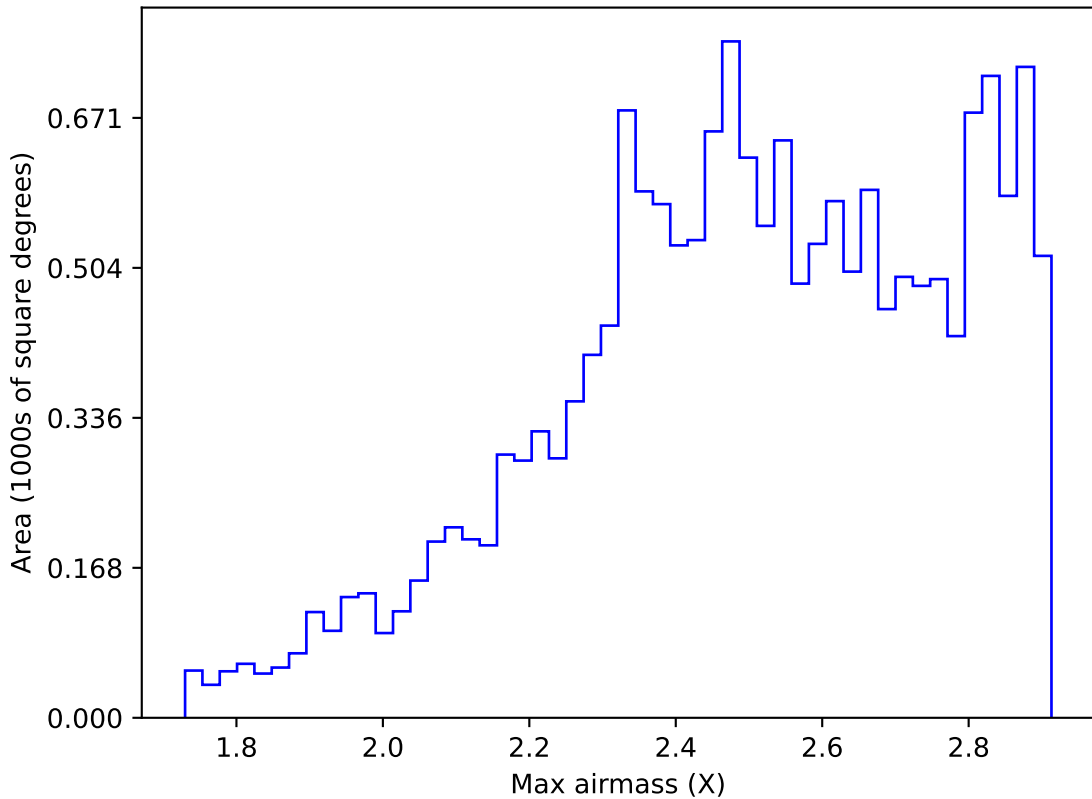
ddf_loaded_fl1_v3.4_10yrs WFD z band: Max airmass
