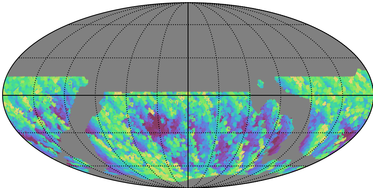
ddf_loaded_fl1_v3.4_10yrs WFD y band: Max airmass
