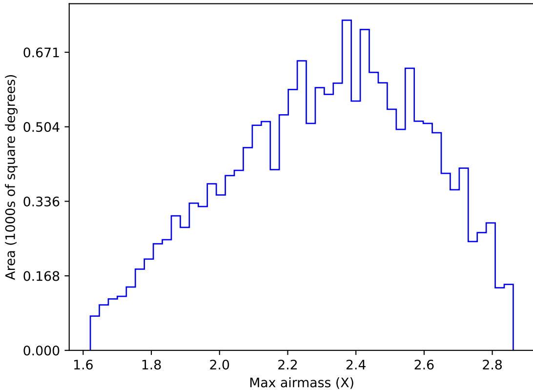
ddf_loaded_fl1_v3.4_10yrs WFD y band: Max airmass
