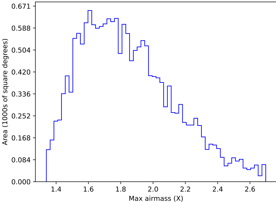
ddf_loaded_fl1_v3.4_10yrs WFD u band: Max airmass
