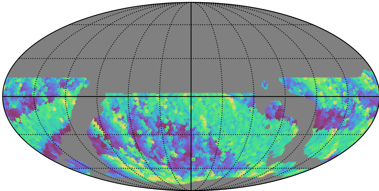
ddf_loaded_fl1_v3.4_10yrs WFD r band: Max airmass
