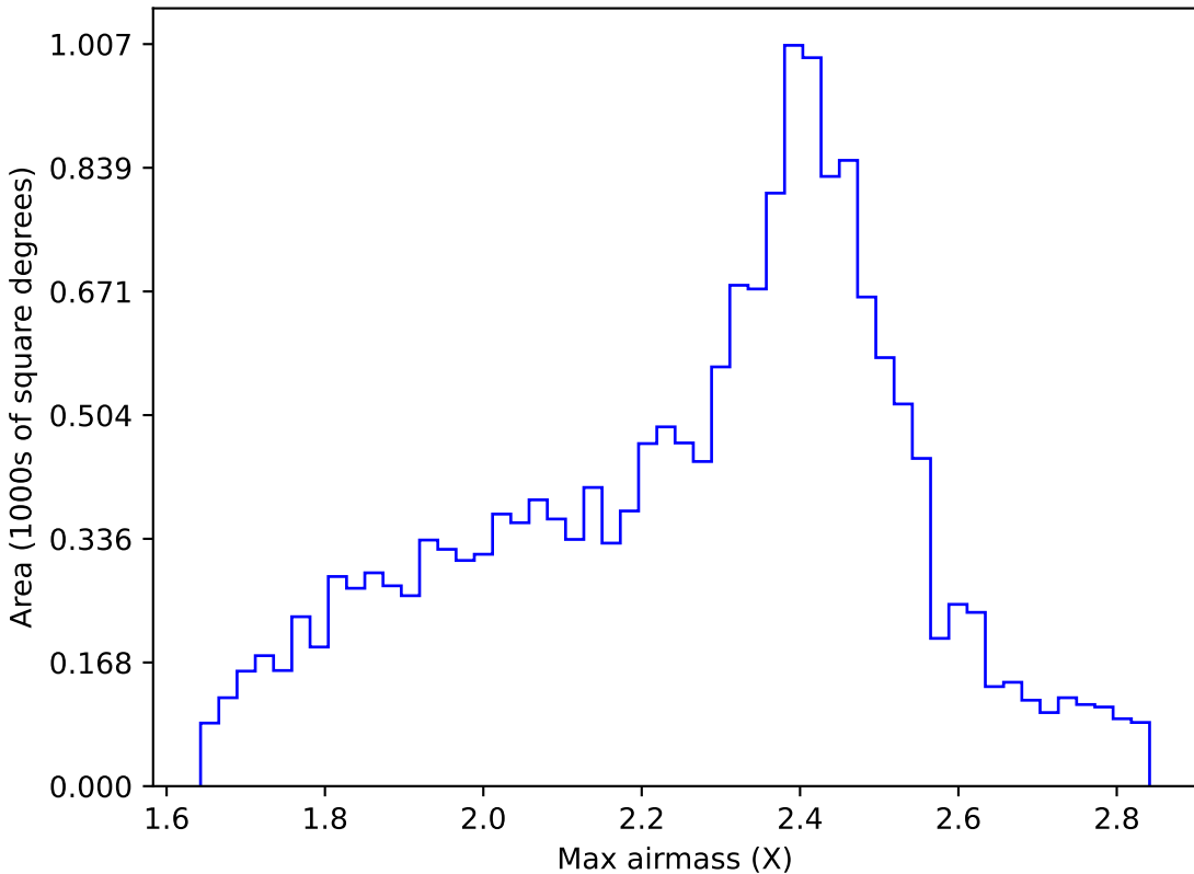
ddf_loaded_fl1_v3.4_10yrs WFD r band: Max airmass
