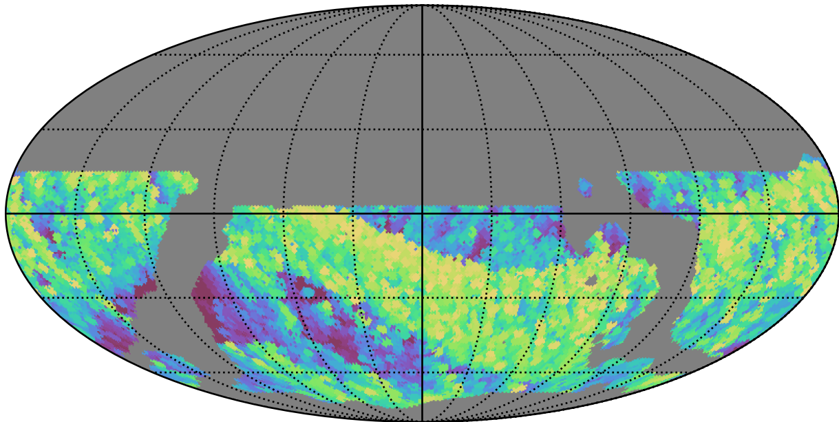
ddf_loaded_fl1_v3.4_10yrs WFD i band: Max airmass
