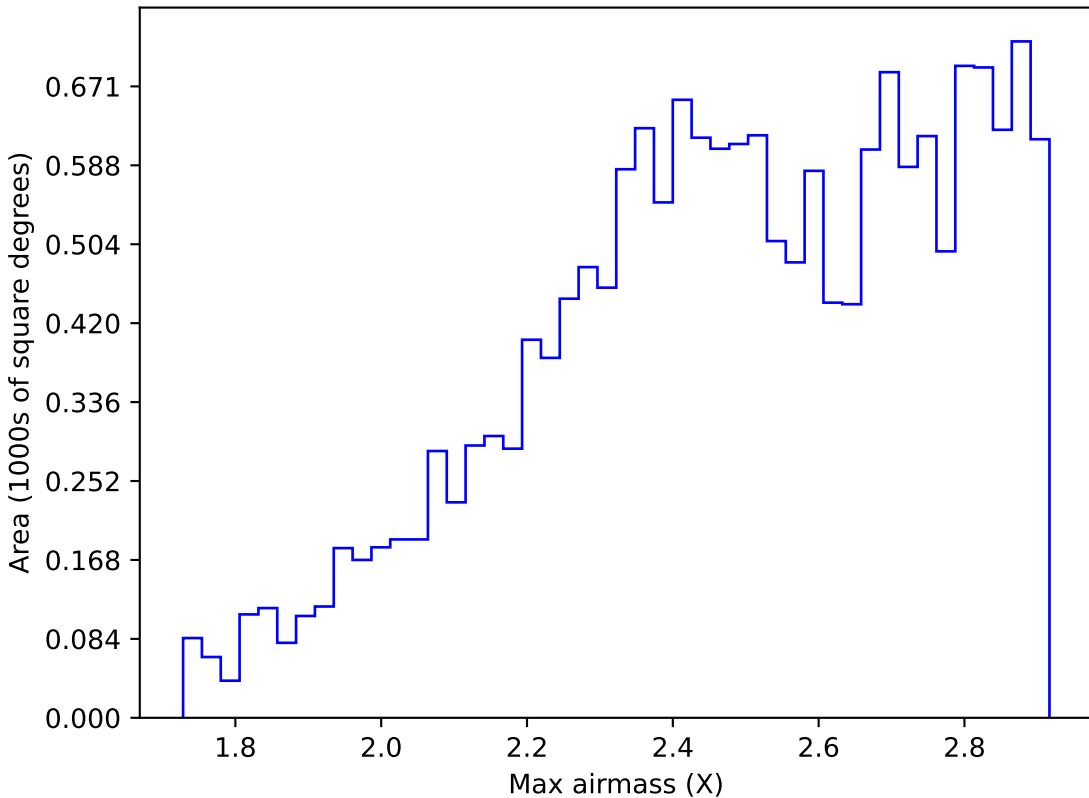
ddf_loaded_fl1_v3.4_10yrs WFD i band: Max airmass
