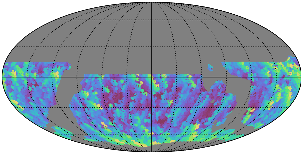
ddf_loaded_fl1_v3.4_10yrs WFD g band: Max airmass
