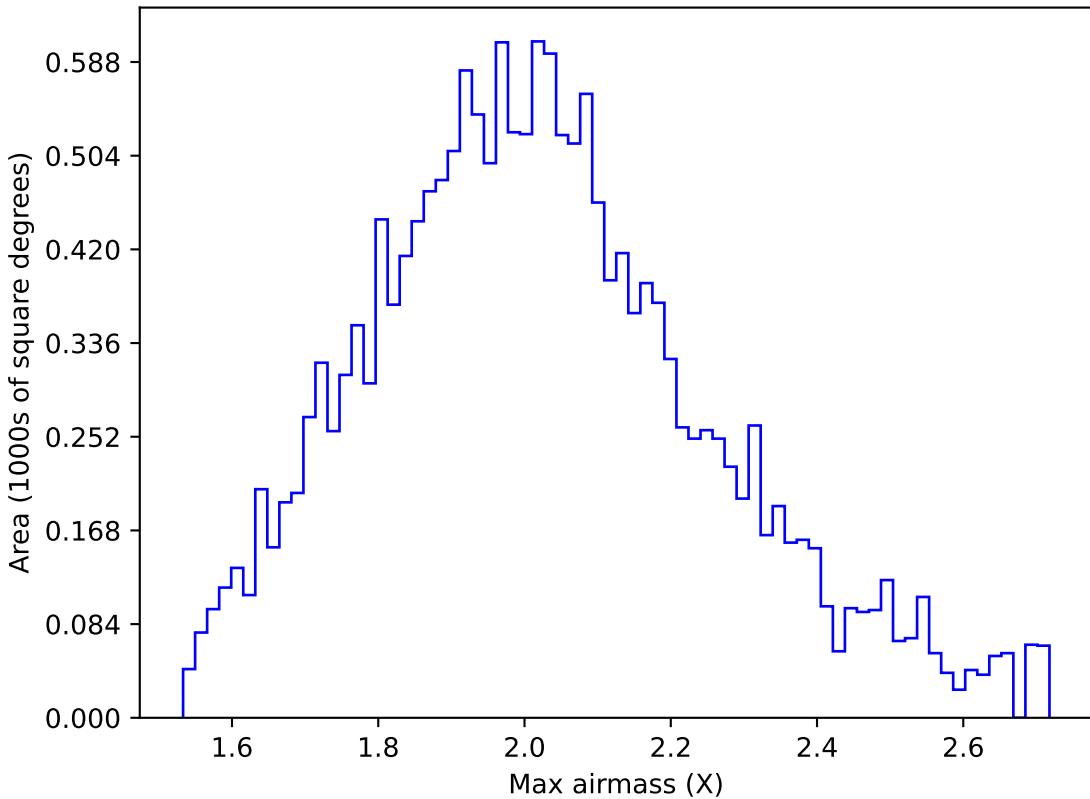
ddf_loaded_fl1_v3.4_10yrs WFD g band: Max airmass
