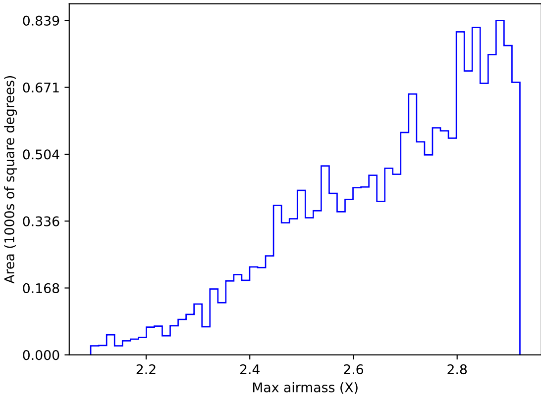
ddf_loaded_fl1_v3.4_10yrs WFD all bands: Max airmass
