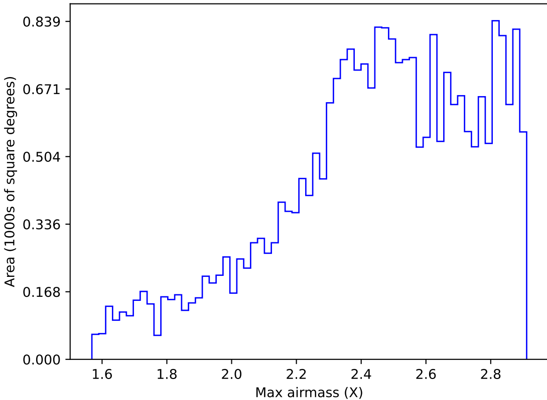
ddf_loaded_fl1_v3.4_10yrs All sky z band: Max airmass
