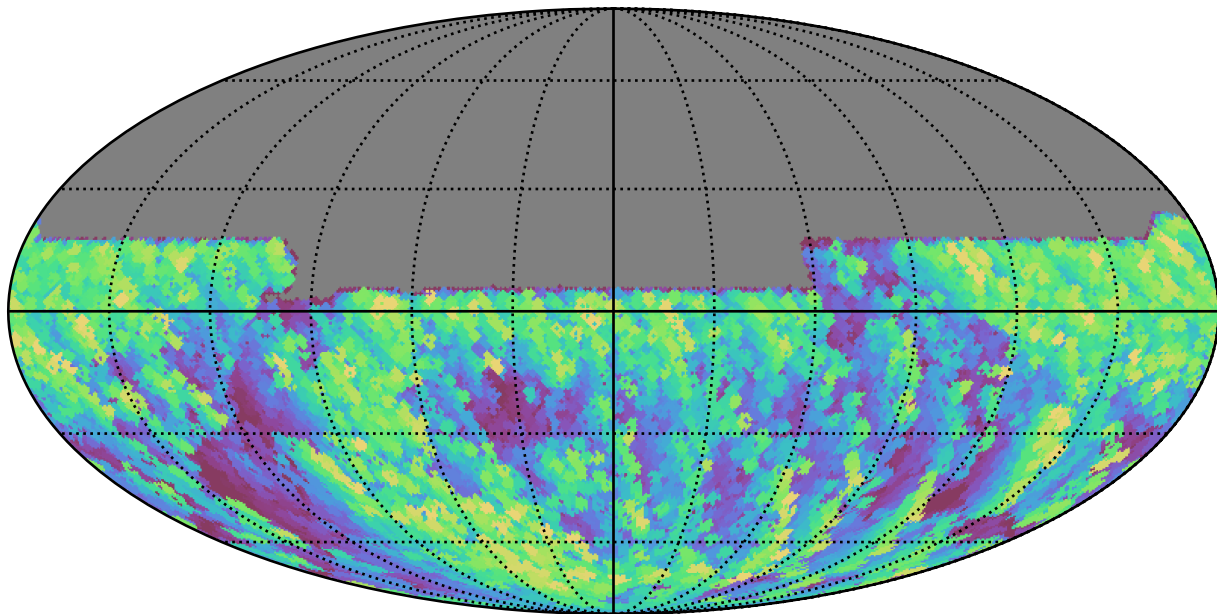
ddf_loaded_fl1_v3.4_10yrs All sky y band: Max airmass
