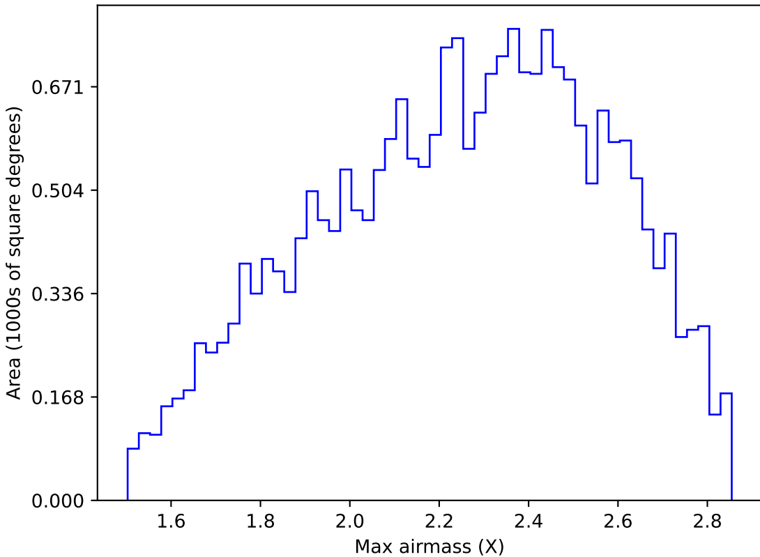
ddf_loaded_fl1_v3.4_10yrs All sky y band: Max airmass
