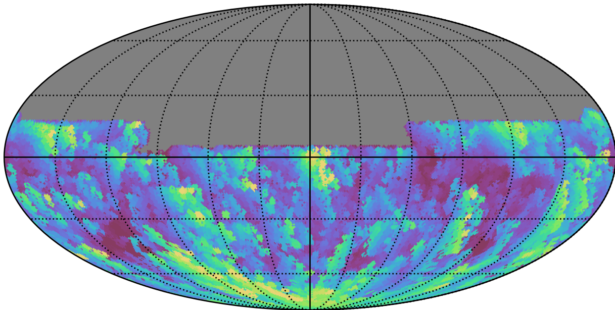
ddf_loaded_fl1_v3.4_10yrs All sky u band: Max airmass
