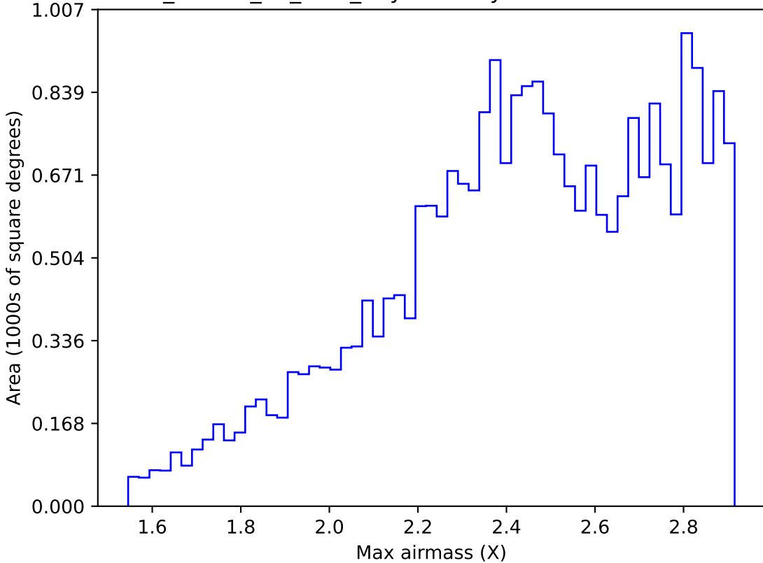
ddf_loaded_fl1_v3.4_10yrs All sky i band: Max airmass
