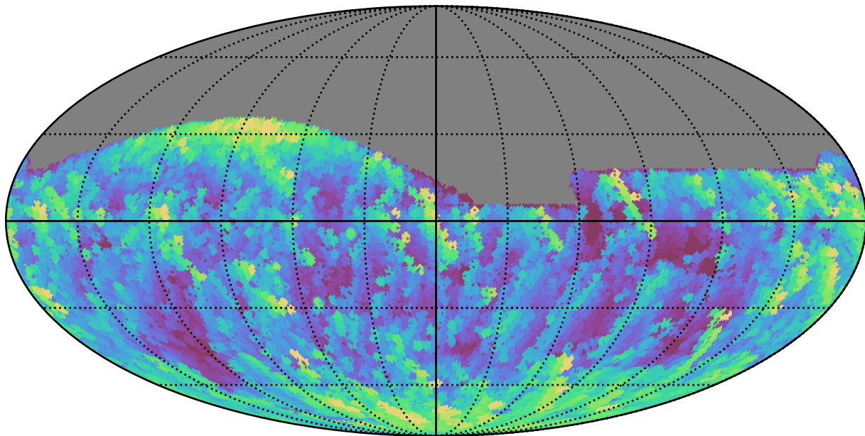
ddf_loaded_fl1_v3.4_10yrs All sky g band: Max airmass
