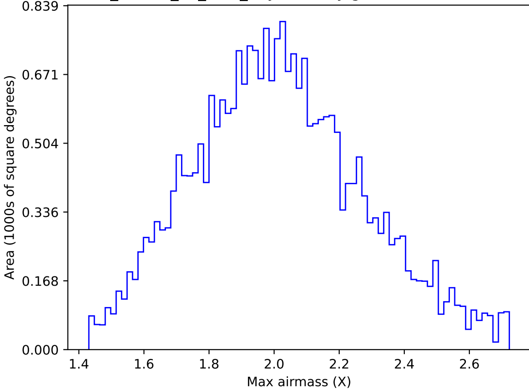
ddf_loaded_fl1_v3.4_10yrs All sky g band: Max airmass
