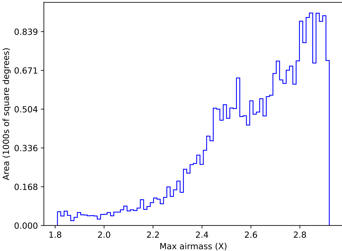
ddf_loaded_fl1_v3.4_10yrs All sky all bands: Max airmass
