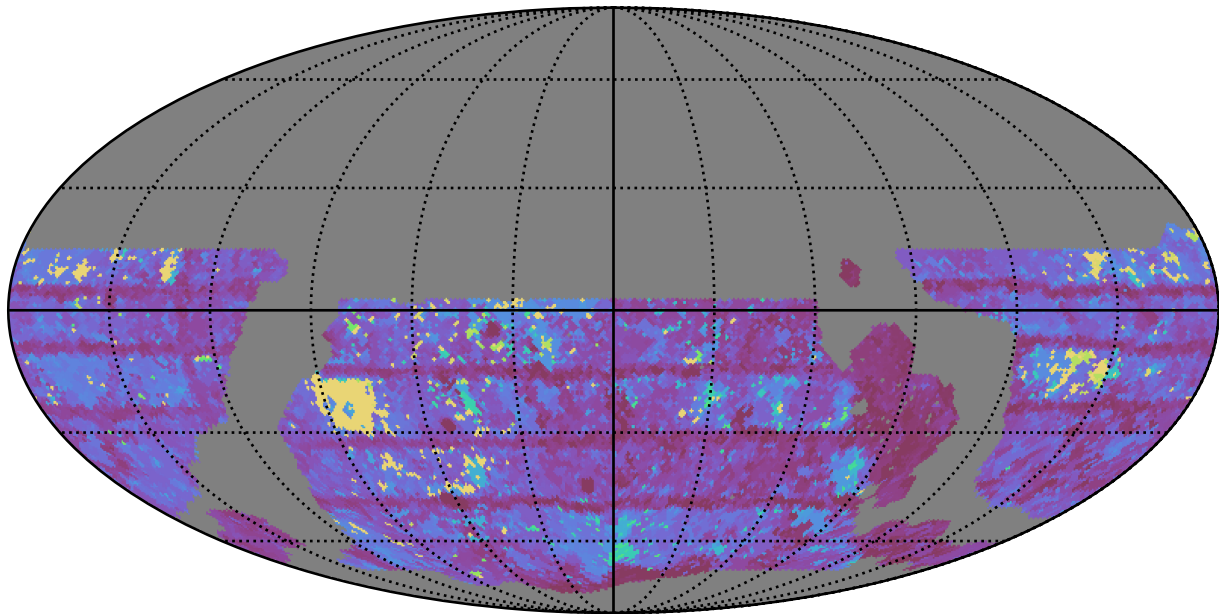
ddf_loaded_fl1_v3.4_10yrs WFD z band: Max Inter-Night Gap
