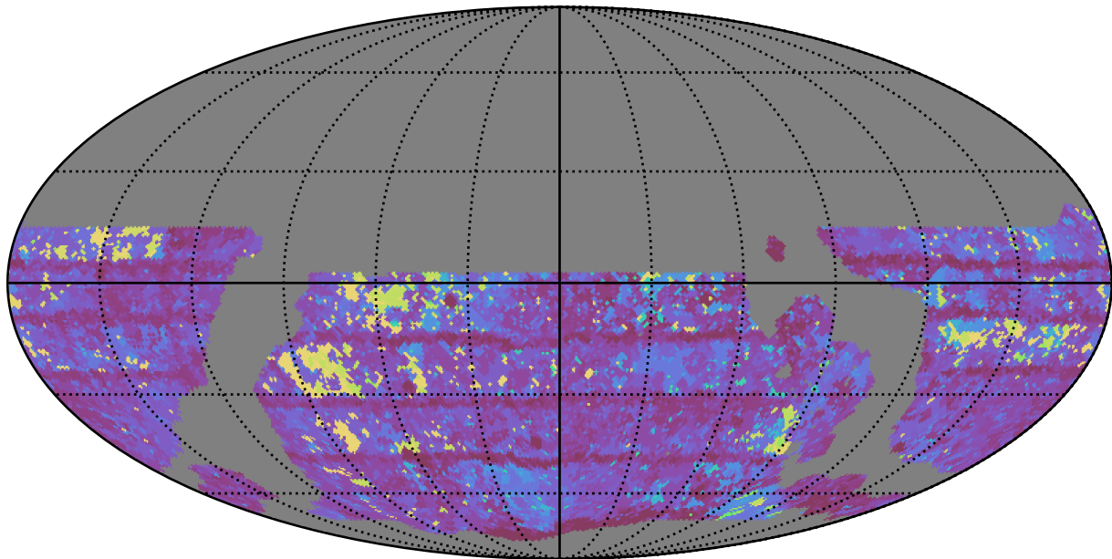
ddf_loaded_fl1_v3.4_10yrs WFD y band: Max Inter-Night Gap
