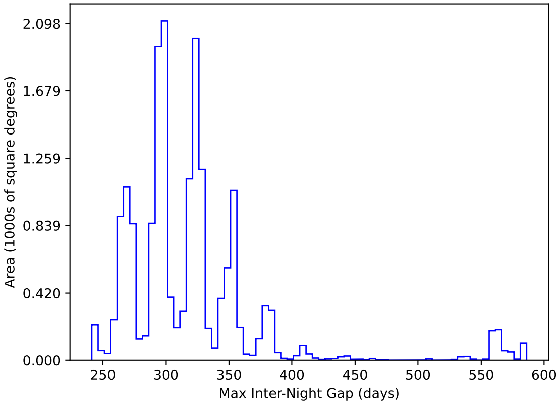
ddf_loaded_fl1_v3.4_10yrs WFD y band: Max Inter-Night Gap
