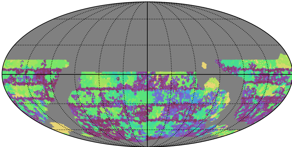
ddf_loaded_fl1_v3.4_10yrs WFD u band: Max Inter-Night Gap
