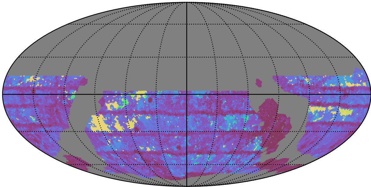
ddf_loaded_fl1_v3.4_10yrs WFD r band: Max Inter-Night Gap
