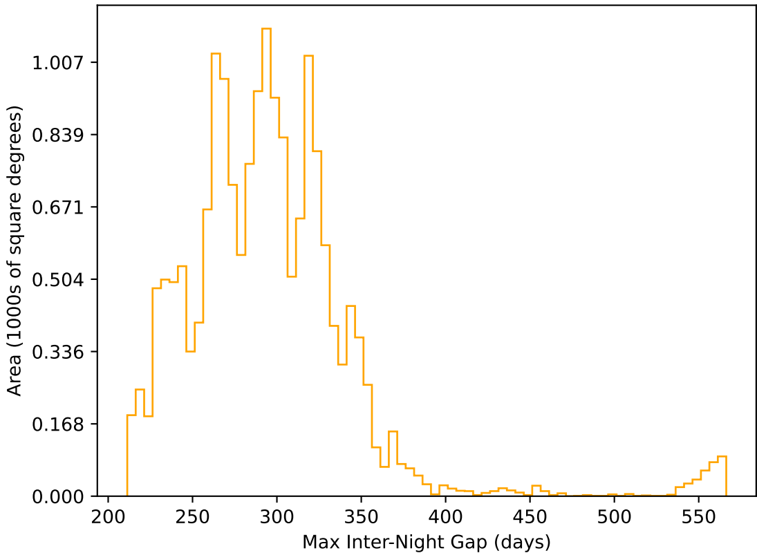
ddf_loaded_fl1_v3.4_10yrs WFD r band: Max Inter-Night Gap
