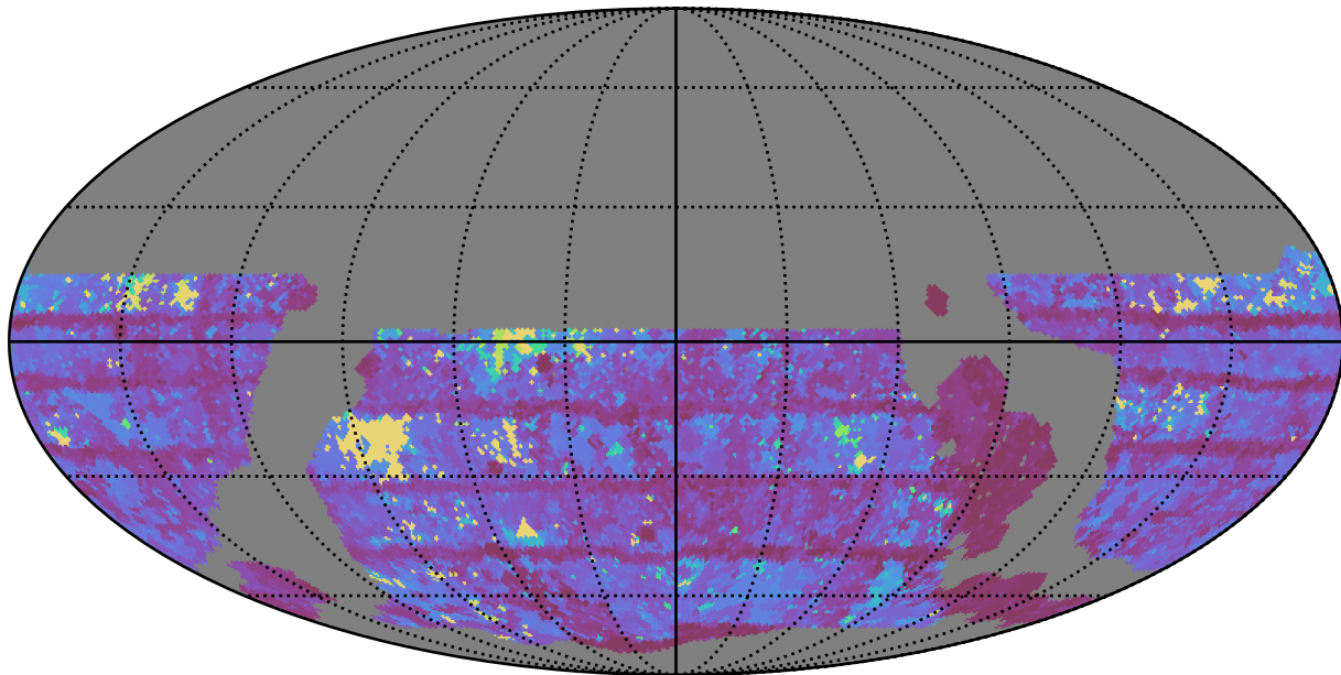
ddf_loaded_fl1_v3.4_10yrs WFD i band: Max Inter-Night Gap
