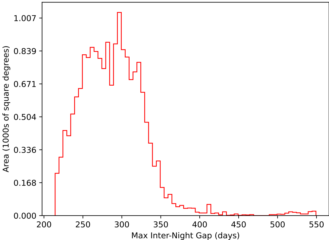
ddf_loaded_fl1_v3.4_10yrs WFD i band: Max Inter-Night Gap
