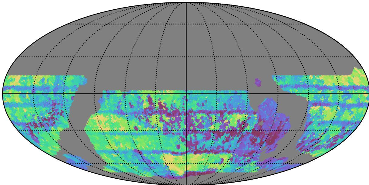
ddf_loaded_fl1_v3.4_10yrs WFD all bands: Max Inter-Night Gap
