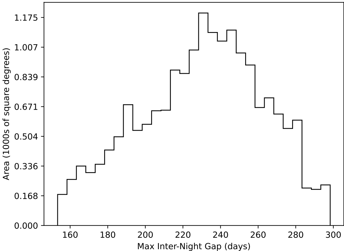
ddf_loaded_fl1_v3.4_10yrs WFD all bands: Max Inter-Night Gap
