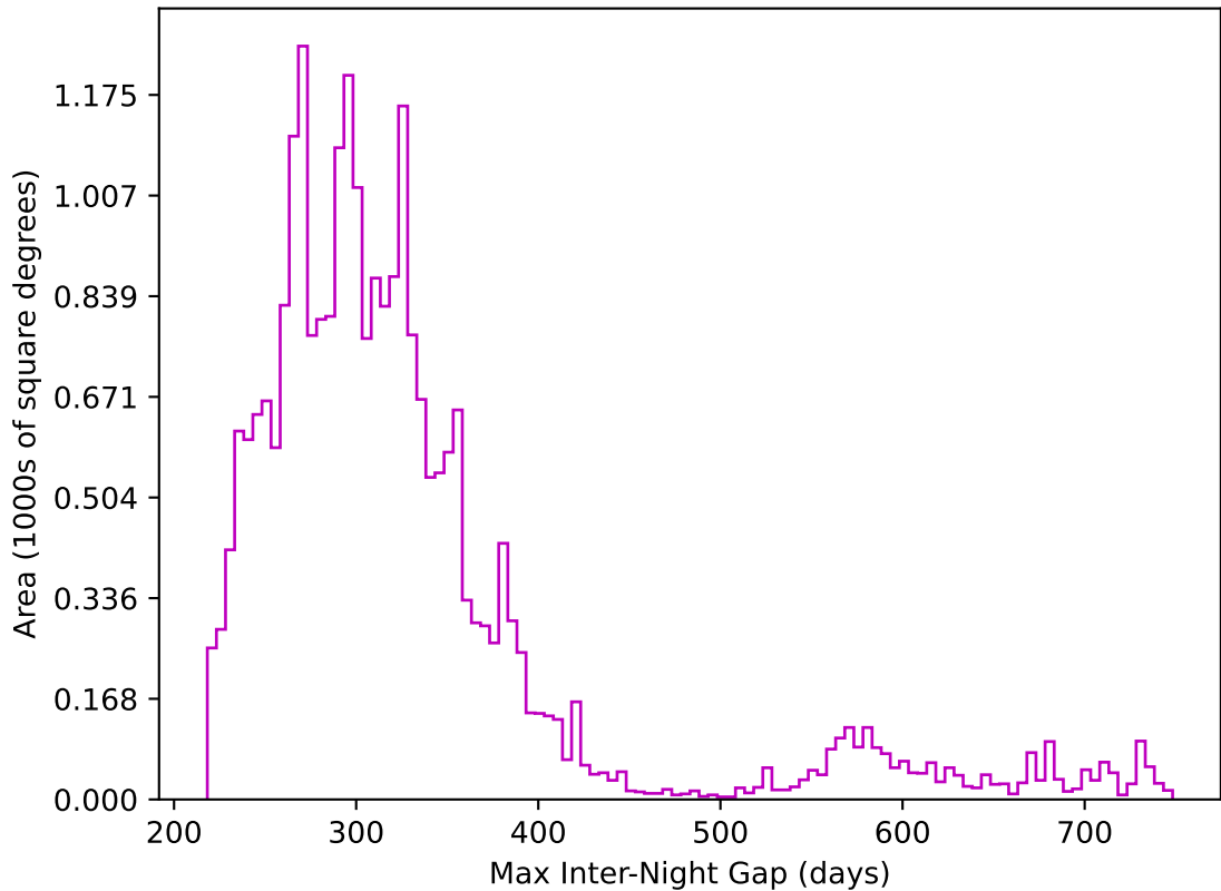
ddf_loaded_fl1_v3.4_10yrs All sky z band: Max Inter-Night Gap
