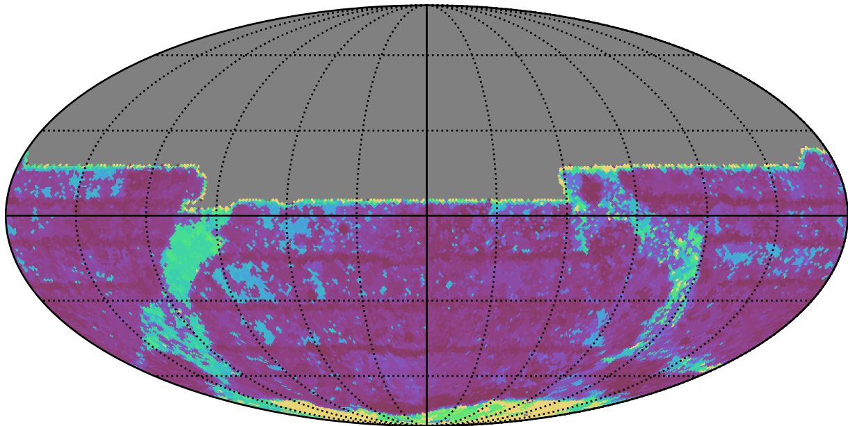
ddf_loaded_fl1_v3.4_10yrs All sky y band: Max Inter-Night Gap
